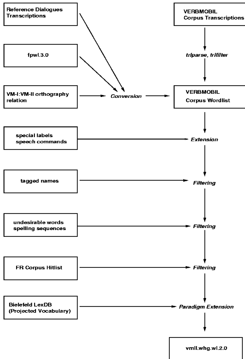
Figure 3: Architecture of the script w1gen
