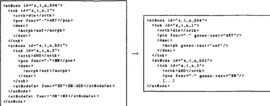
Figure 1. An example from the TüBa-D/Z treebank (represented in the Tuszelda format) before (left) and after processing the resource with our normalisation tools (right)
