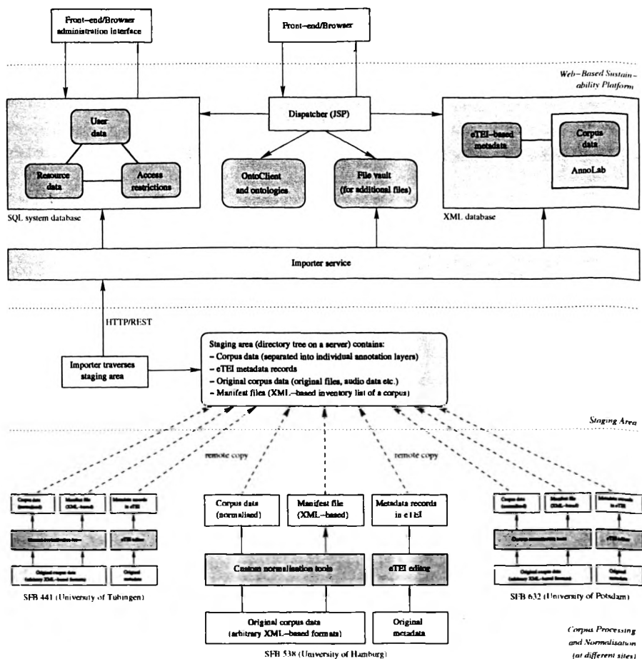
Figure 2. Resource normalisation, the staging area and the primary SPLICR components
