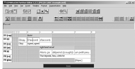
Figure 4: EXMARaLDA Partitur-Editor
