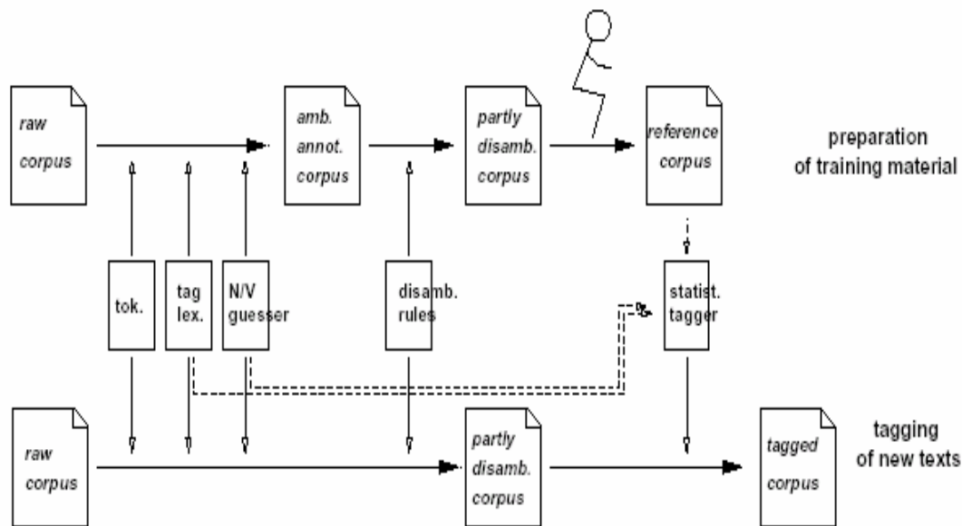
Figure 1: Architecture for the creation of training material and for the tagging of new texts
